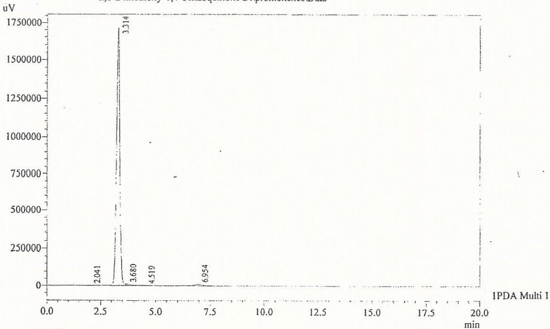
Chromatogram 2,6-Dimethoxy-1,4-benzoquinone D:\promonence\Data
